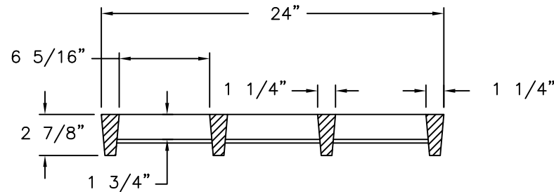
GRATE SECTION
