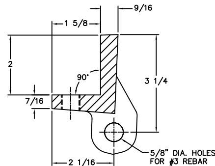
FRAME SECTION
